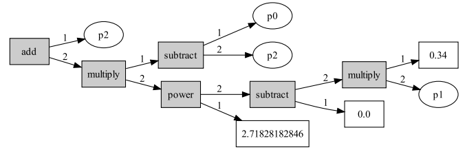
Fig. 6. Tree representation of the first ( F_1 ) of two functions that determine a simplified response facial expression to the causing event. The tree represents the initial exponential guess for the first component ( F_1 ) of the response function. The evolutionary optimisation takes place by introducing mutations of this tree until the response functions are found.
